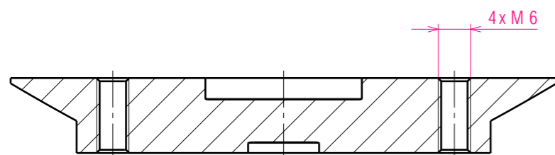
Cut B-B
